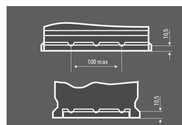
Base holddown
