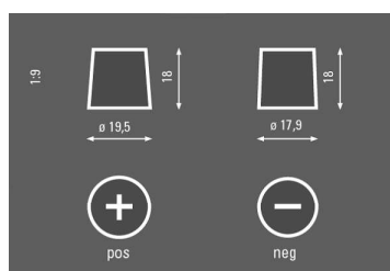
Terminal Type
